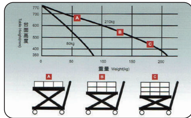
承重高度對應圖 Load and Height Chart (Model APL21)
